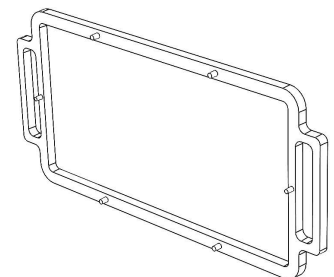
Spacer for 1/2" drawer box.
